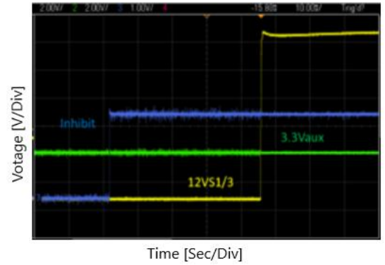
Figure 3.5.2.4-2. Enable Turn-on, 12V first
