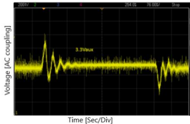
Figure3.5.2.6-2. 3.3V Dynamic Response
